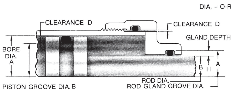
Illustration of Industrial O-Ring Application
